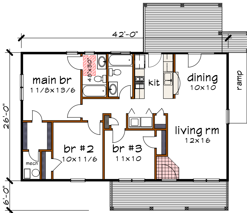
Floor 1 plan
