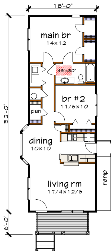
Floor 1 plan
