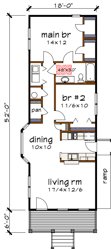
Floor 1 plan
