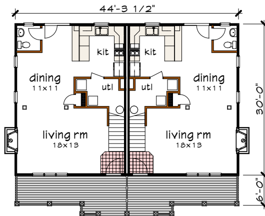
Floor 1 plan
