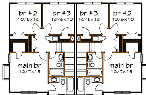
Floor 2 plan
