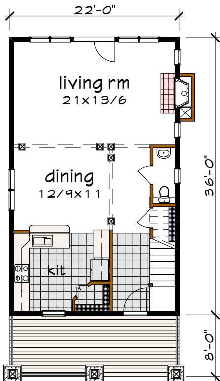
Floor 1 plan
