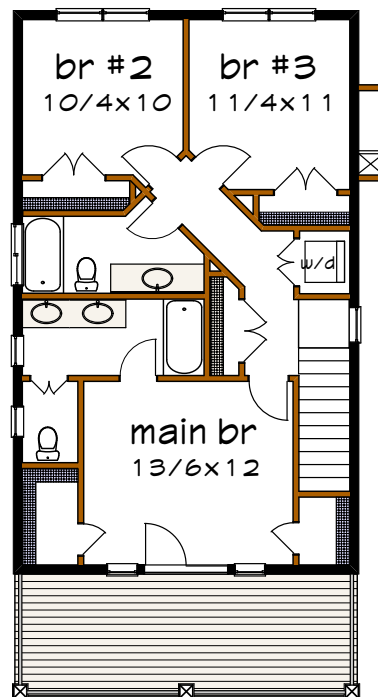
Floor 2 plan
