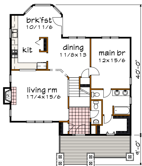
Floor 1 plan
