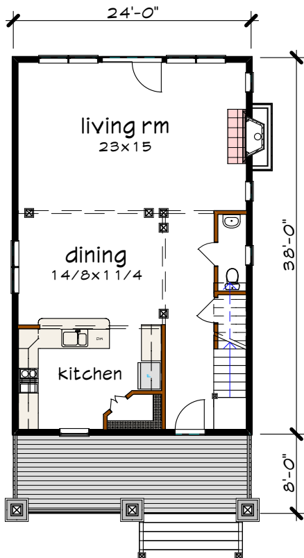
Floor 1 plan
