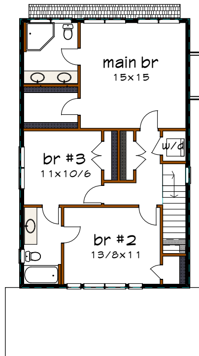
Floor 2 plan
