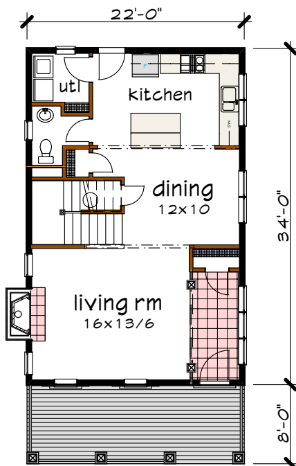
Floor 1 plan
