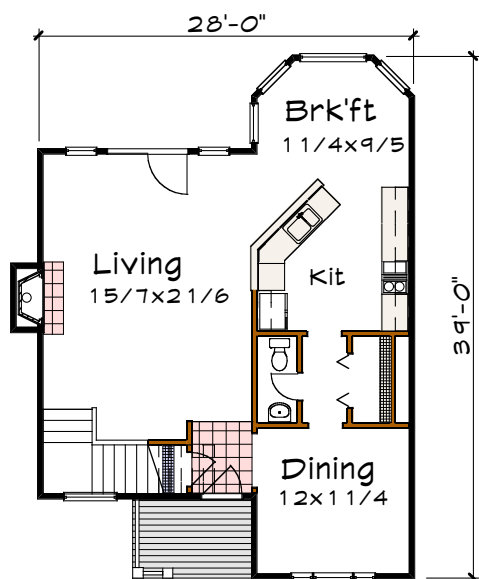
Floor 1 plan
