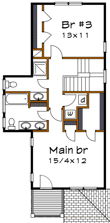
Floor 2 plan
