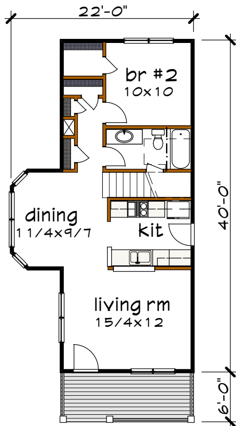
Floor 1 plan
