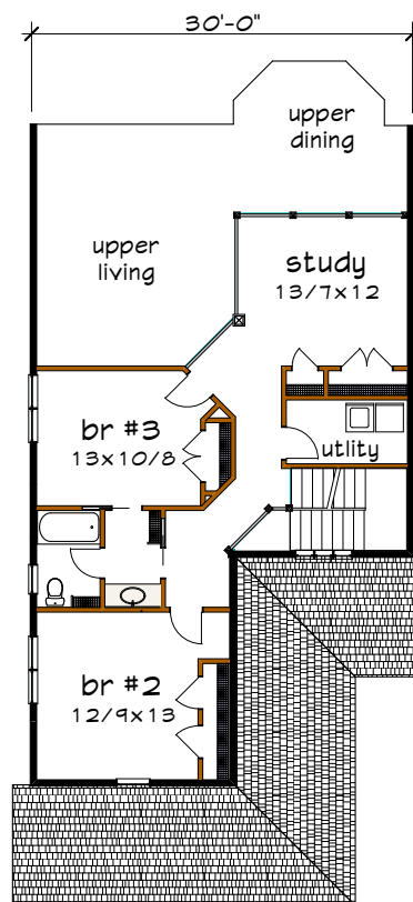
Floor 2 plan
