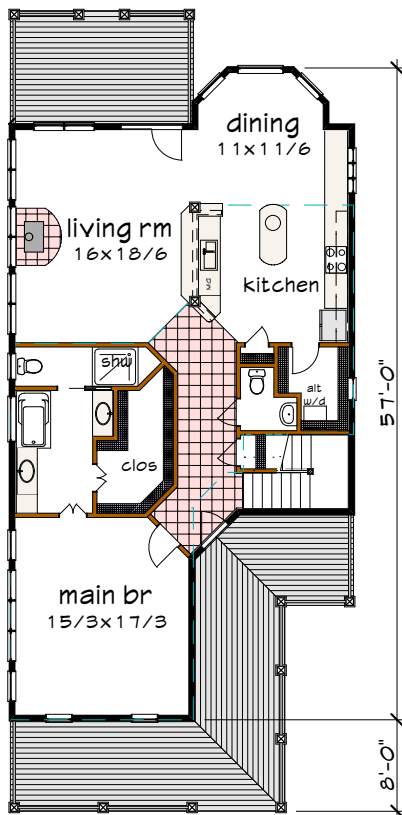
Floor 1 plan
