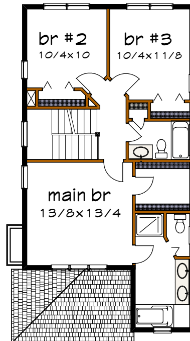
Floor 2 plan
