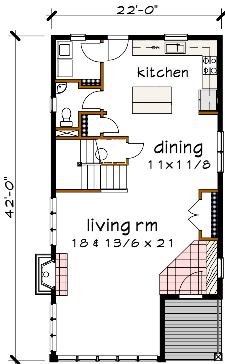
Floor 1 plan
