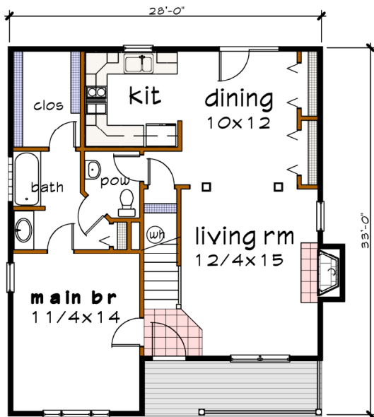
Floor 1 plan
