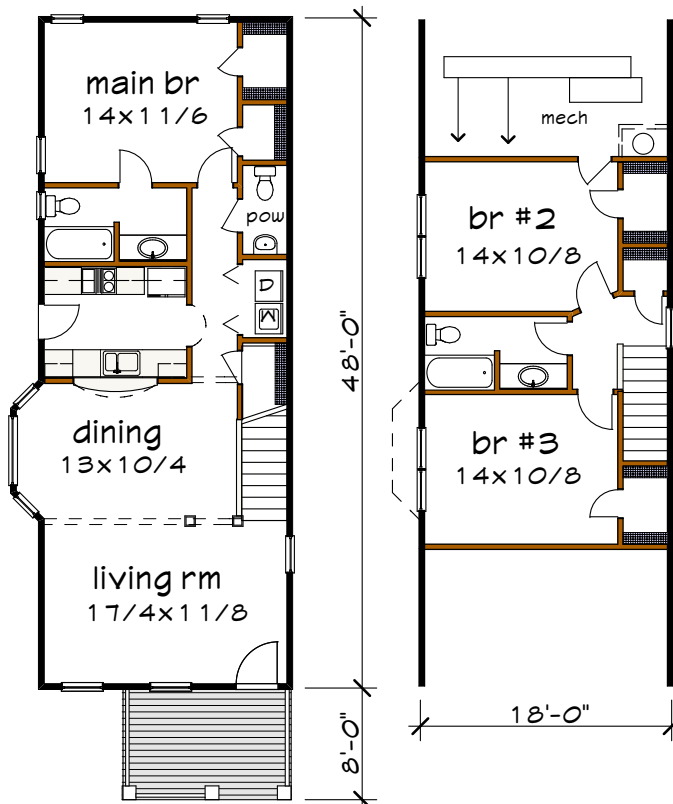
Floor 1 plan Floor 2 plan
