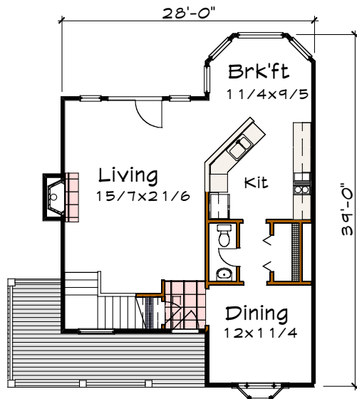
Floor 1 plan
