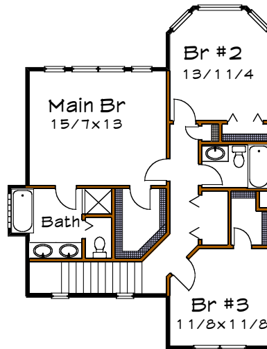
Floor 2 plan
