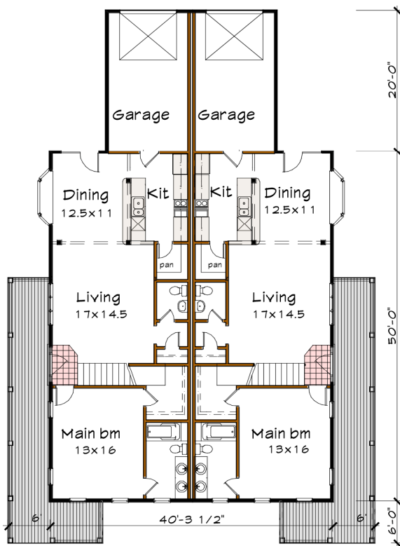
Floor 1 plan
