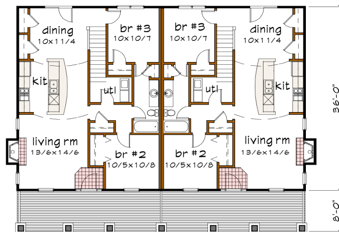
Floor 1 plan
