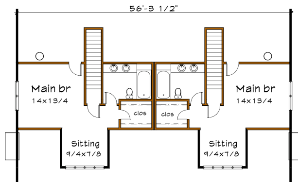
Floor 2 plan
