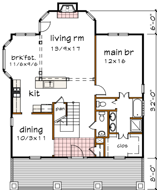
Floor 1 plan
