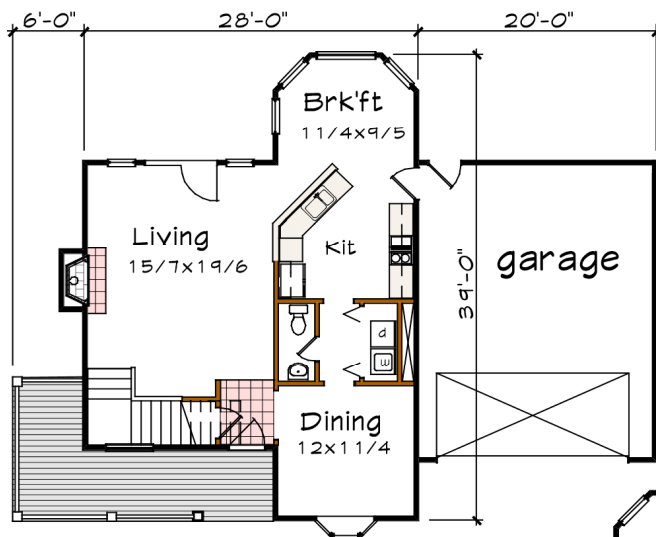
Floor 1 plan
