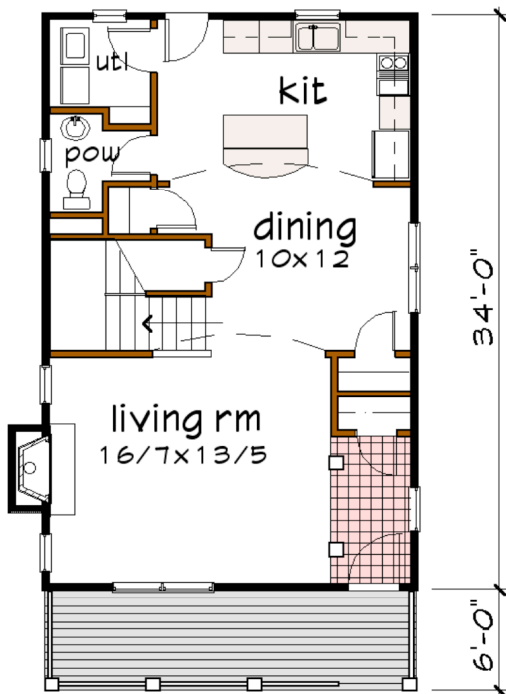
Floor 1 plan
