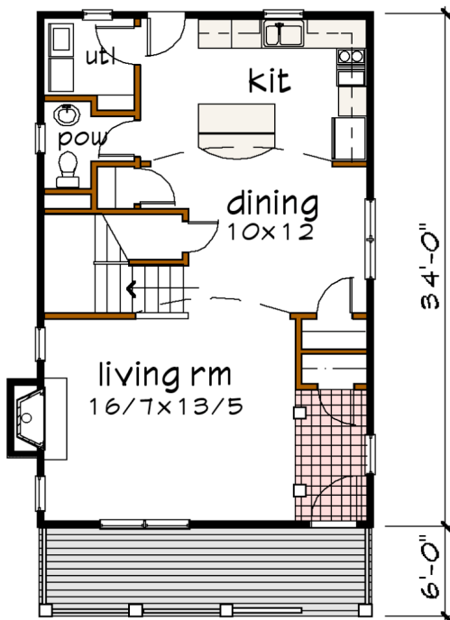
Floor 1 plan
