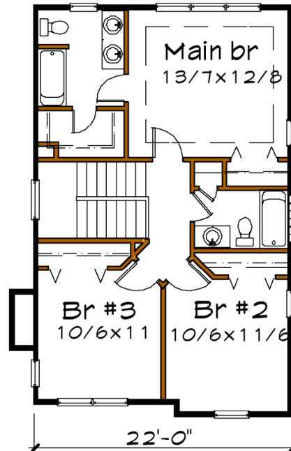
Floor 2 plan
