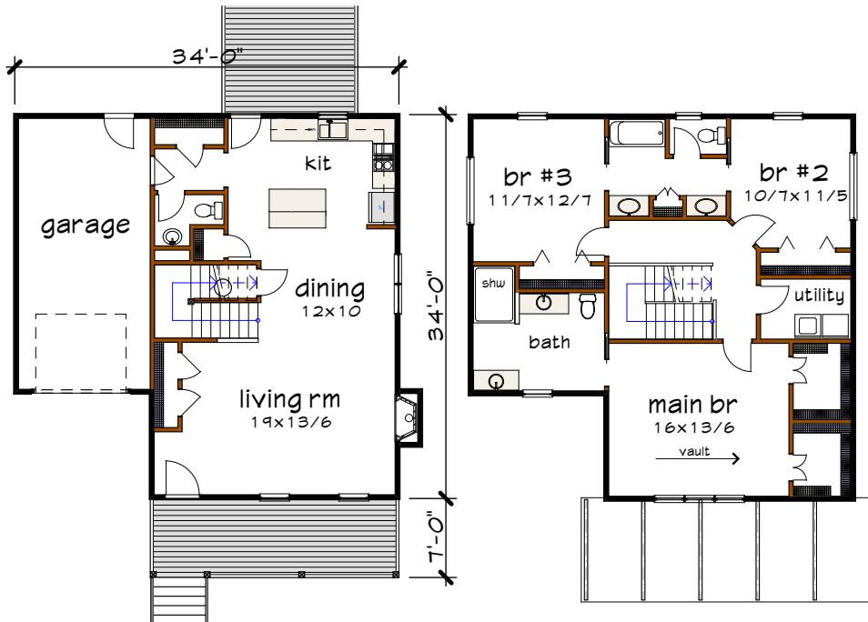
Floor 1 plan
