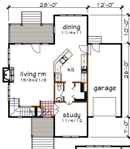
Floor 1 plan
