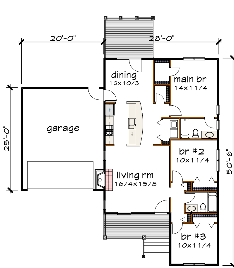
Floor Plan
