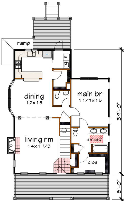
Floor 1 plan
