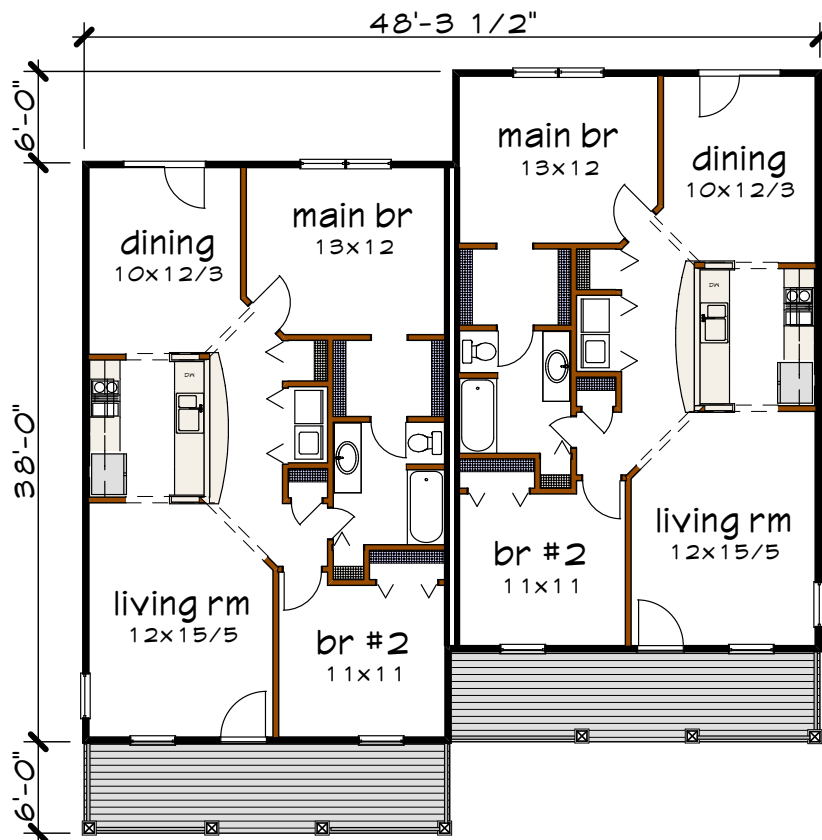
Floor plan
