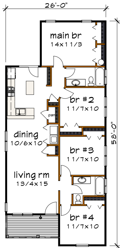
Floor 1 plan
