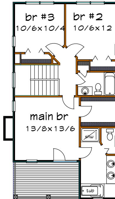
Floor 2 plan
