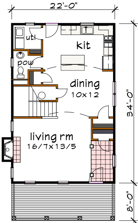
Floor 1 plan
