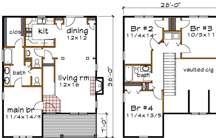
Floor 1 plan
