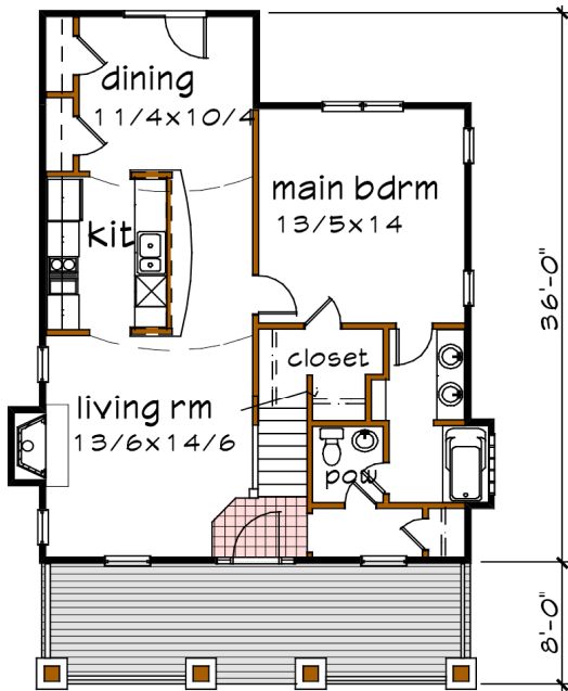
Floor 1 plan
