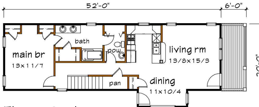
Floor 1 plan
