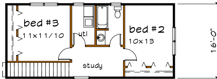
Floor 2 plan
