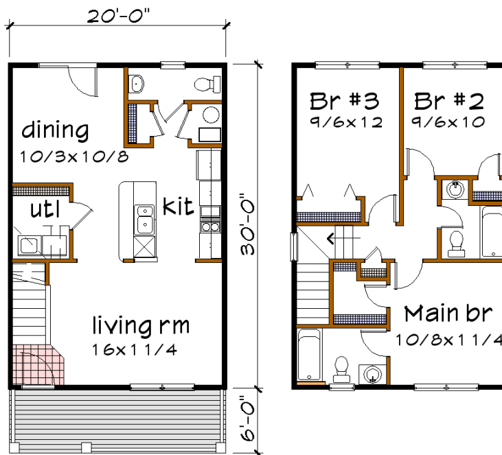
Floor 1 plan
