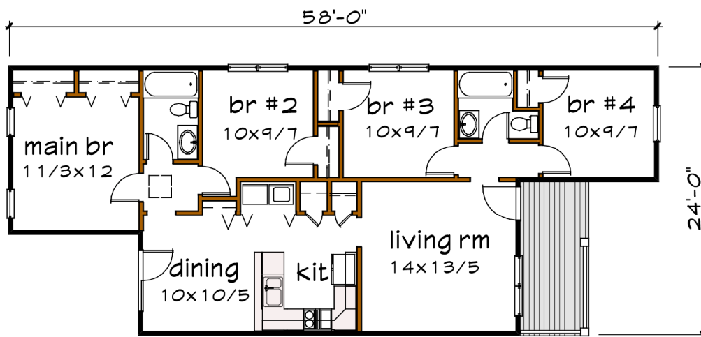
Floor 1 plan
