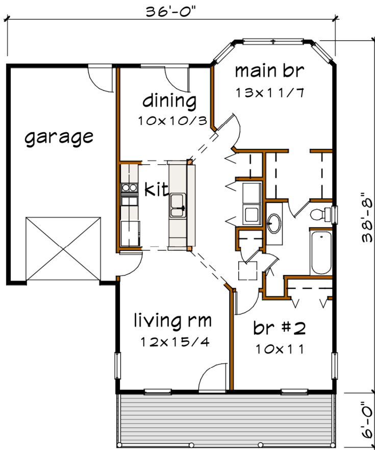
Floor 1 plan
