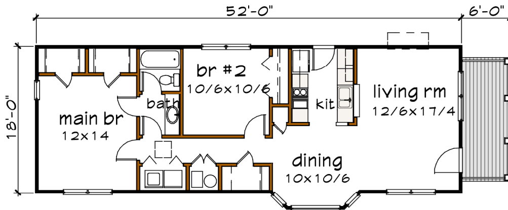
Floor 1 plan
